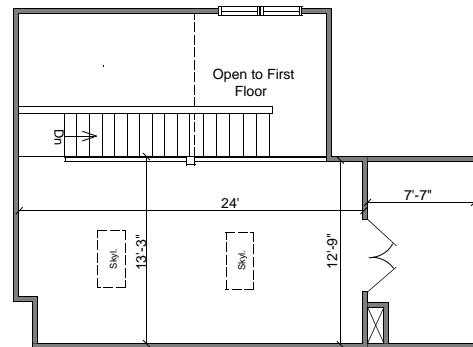
SECOND FLOOR 431 SQ. FT.
