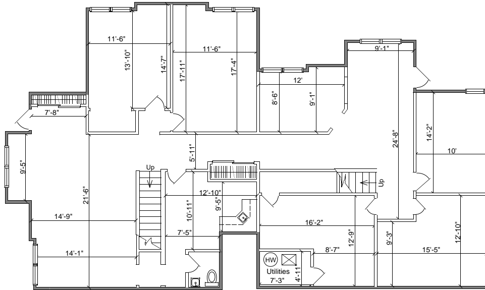
FIRST FLOOR 2,154 SQ. FT.
