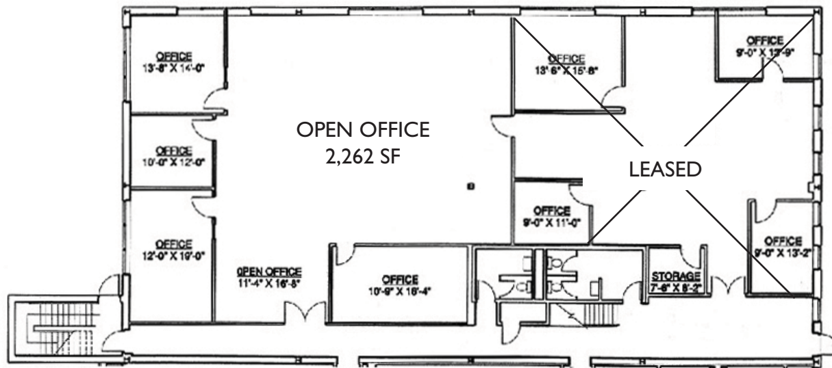
SUITE "A-1" FIRST FLOOR PLAN A north arrow is located to the left of the scale bar. The scale bar is marked with 0, 5, 10, and 20 feet.
